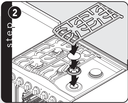
Burner heads and burner caps are packed in the cardboard top pack with the grates. Align burner head on burner base. Place burner cap on burner head. Place grate onto the burner pan.
