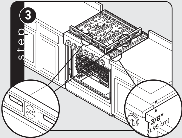
Check that unit is level side to side and front to back. The side trim must be 3/8" (0.95 cm) above countertop. If unit is not level, repeat Steps 5-7 in "Leveling/Adjustments/Alignment" section.
