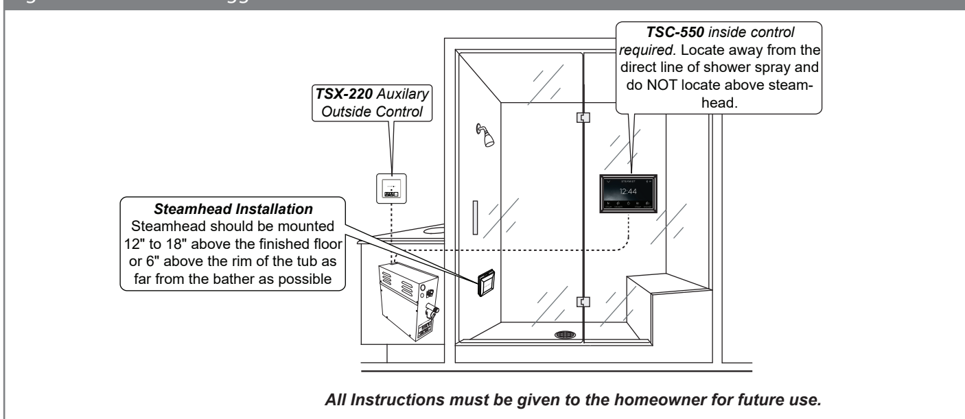
Figure 4 - Installation Suggestions
