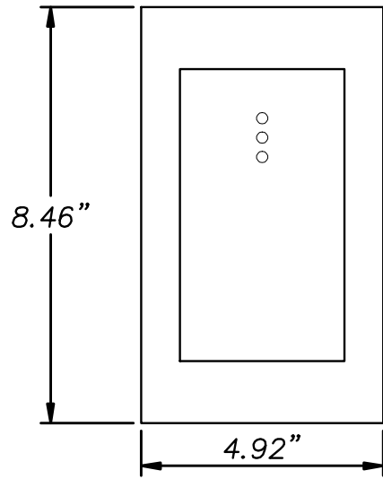
Back plate
