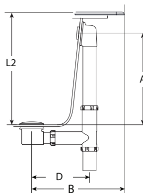
Drain/Overflow
