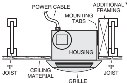
HOUSING MOUNTED TO "1" JOIST Requires additional framing for mounting tabs.
